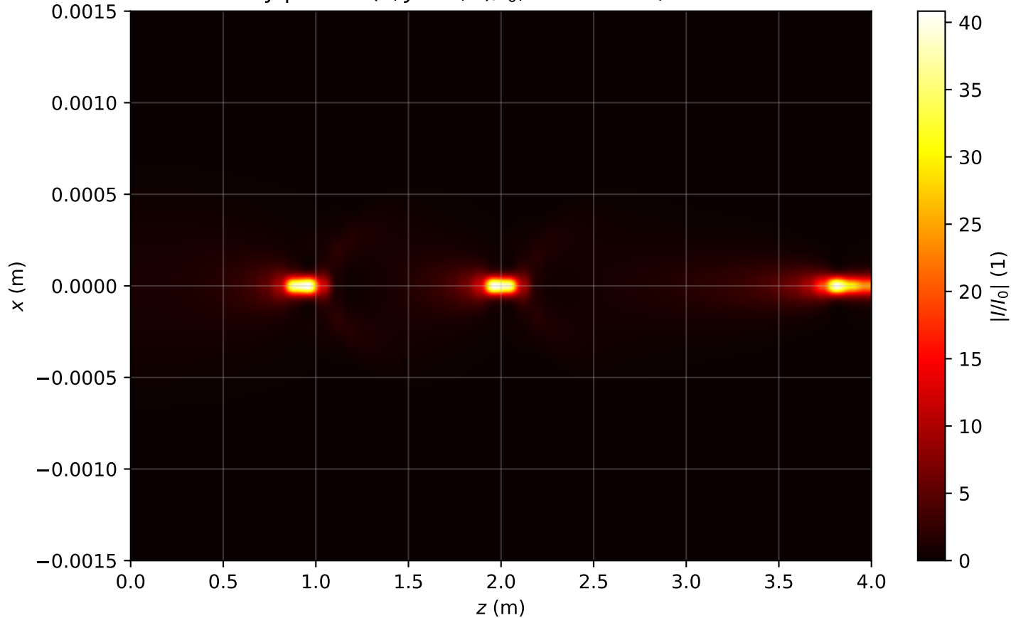
Intensity profile I(x, y = 0, z)/I_0 , P_{in}=2.5P_{cr} , artificial time
